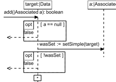
Figure 6. Interaction Res. Plain/OneOpposite
