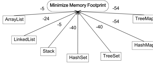
Figure 7. Memory Usage in Bytes and Corresponding Impact Model
