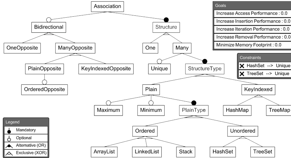
Figure 1. Screenshot of Variation Interface of the Association Concern
