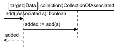
Figure 4. Base Behaviour of add
