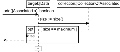
Figure 5. Aspect Sequence Diagram Maximum
