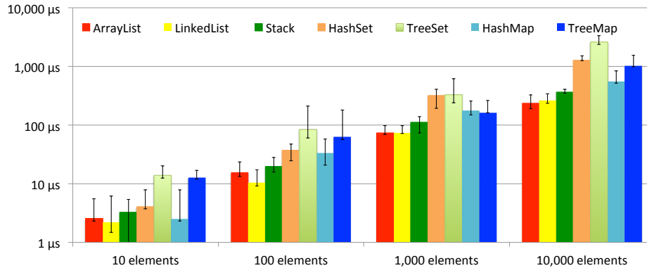
Figure 8. Insertion Performance of Different Collection Implementations
